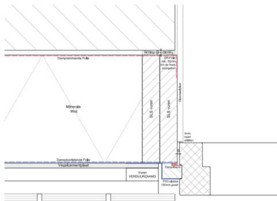
DETAIL 5a
