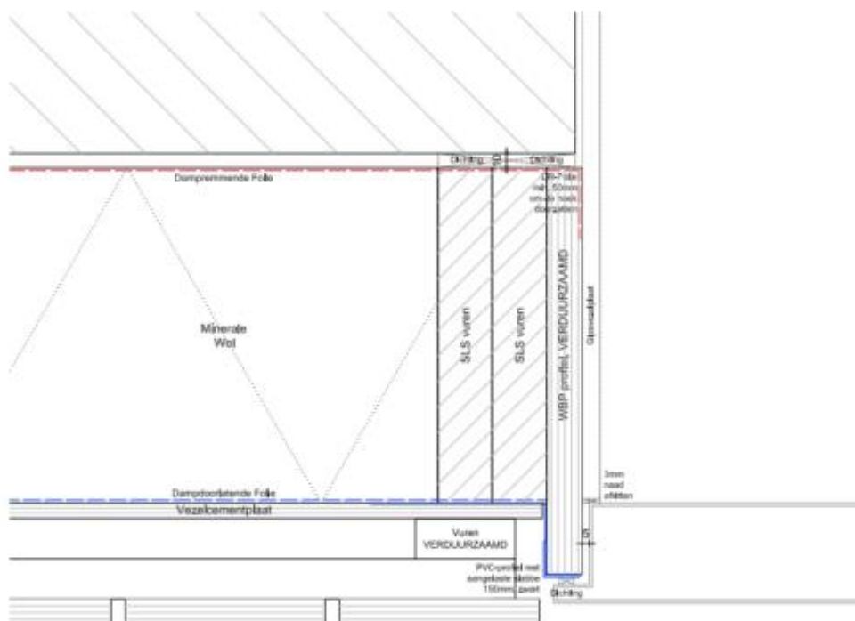
DETAIL 5b
